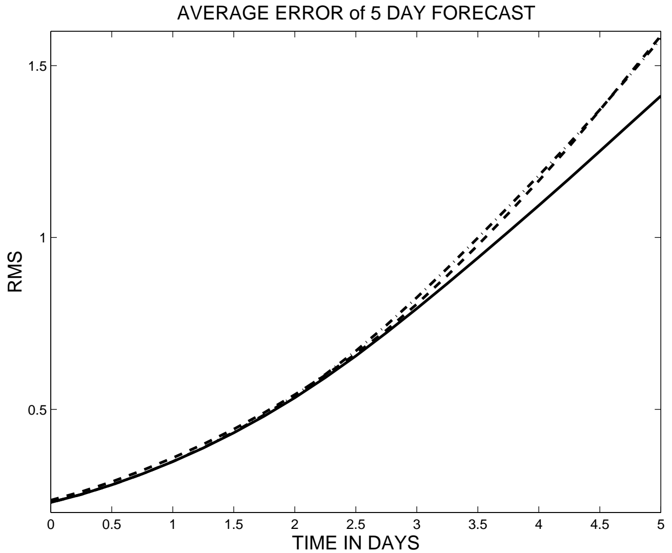
Figure 2. Mean forecast errors as function of forecast time for 4D-VAR with 96 hour (dashed) and for a 4D-LETKF with 24 hour analysis window using an ensemble forecast (solid) and forecast from the mean analysis state (dot-dashed). The mean analysis error of each scheme is at time 0.
