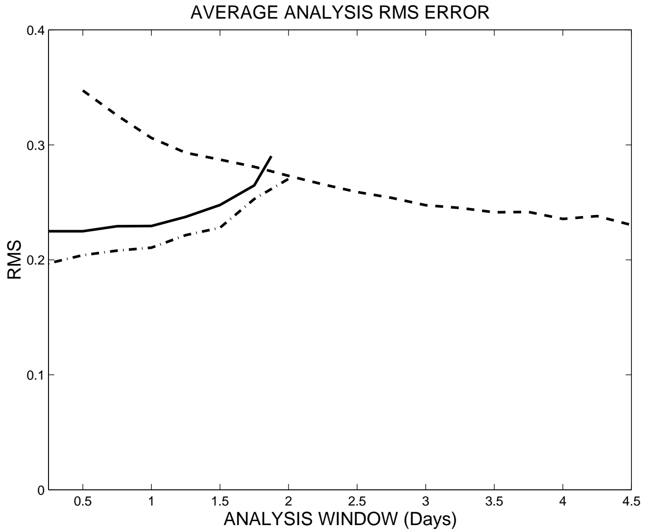
Figure 1. We show the mean analysis error as a function of analysis window for 4D-VAR (dashed). The mean analysis error is shown as a function for time between analyses for 4D-LETKF with 15 ensemble members and localization (solid) and 50 ensemble members and no localization (dot-dashed). The 15 (50) ensemble member 4D-LETKF experiments used inflation factors of 10% (8%) for the 12 hour, n = 8 , analysis window, 23% (14%) for the 24 hour, n = 16 , analysis window, and 65% (24%) for the 42 hour, n = 28 , analysis window. The 4D-LETKF analysis diverged for all inflation factors below 100% for analysis windows longer than 42 hours and 48 hours in the 15 and 50 ensemble member experiments, respectively.
