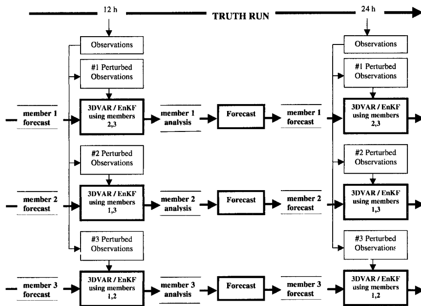
FIG. 2. Illustration of cycle used in generating hybrid analyses for a hypothetical three-member ensemble. Each member receives a different set of perturbed observations. Ensemble-based covariances are estimated using fellow members but excluding the member currently being processed.
