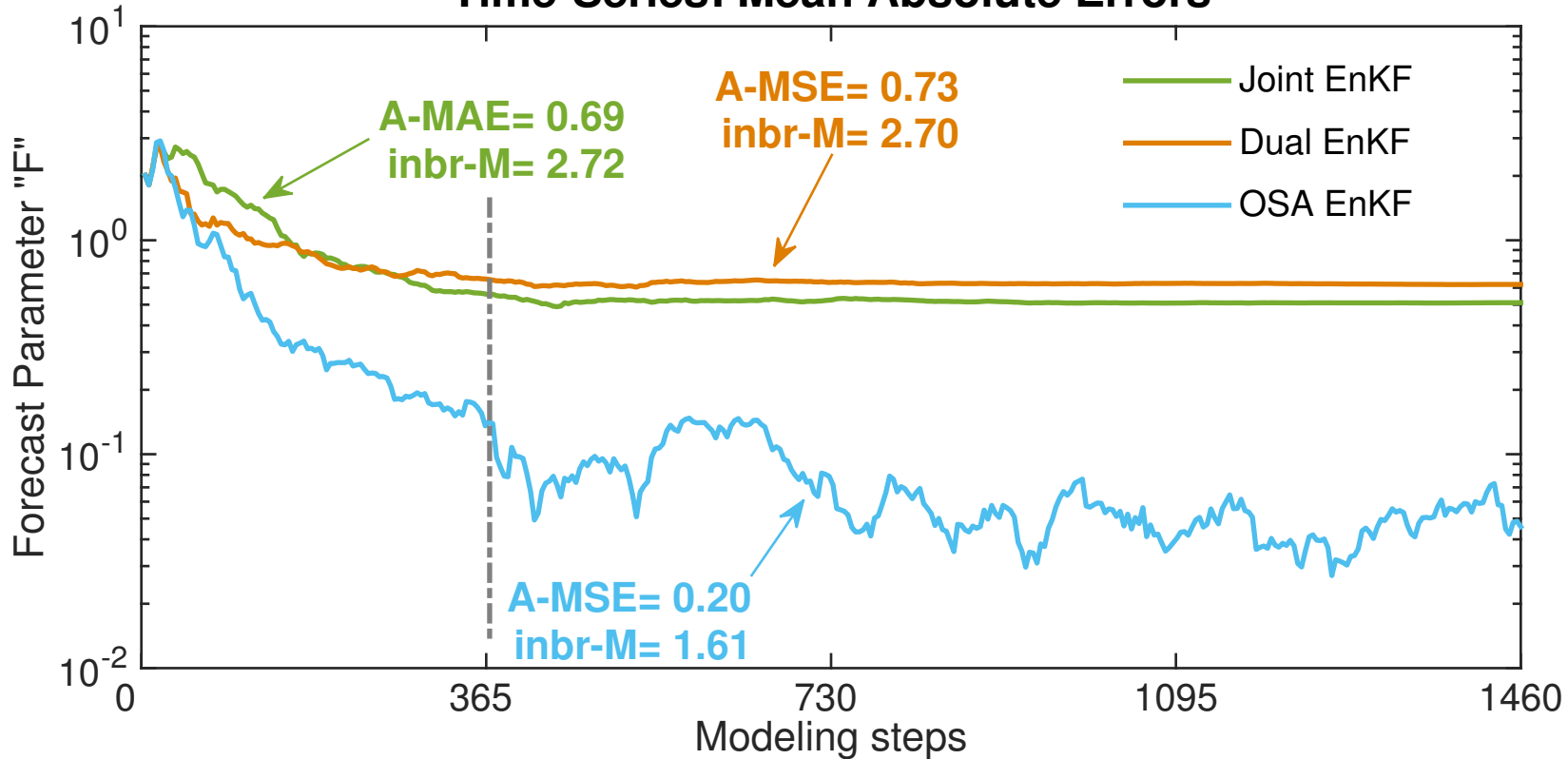
Time-Series: Mean Absolute Errors
